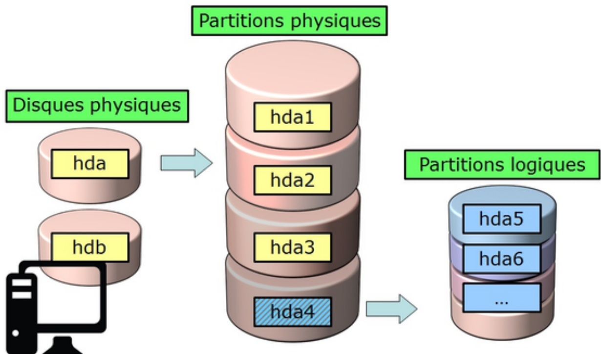
Figure 12. Identification des partitions
