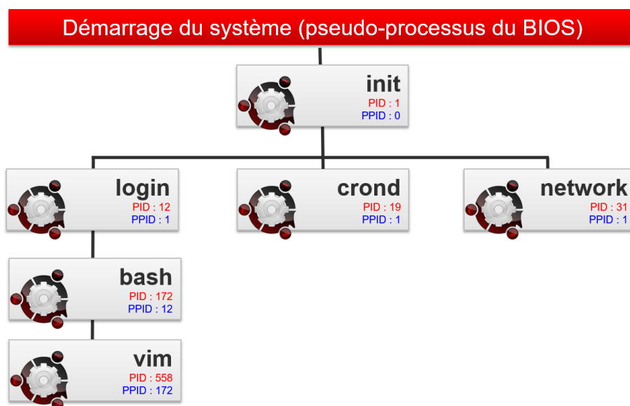
Figure 28. Filiation des processus
