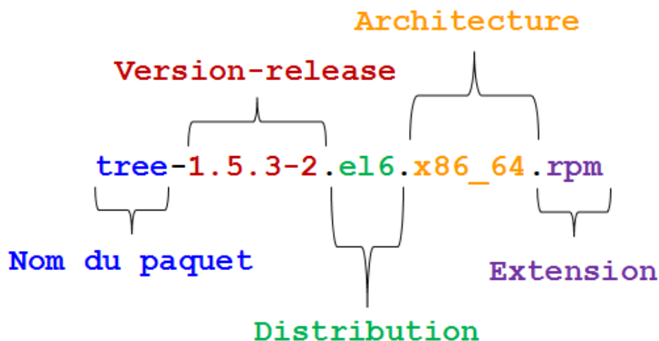
Figure 36. nom-version-edition.architecture.rpm
