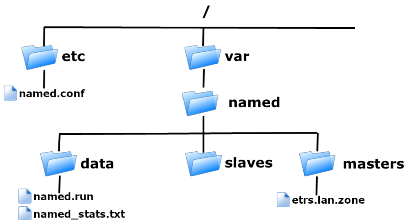
Figure 41. Arborescence du service Bind
